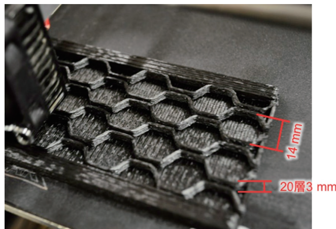
Figure 2 Honeycomb structure molded by composite 3D printer
