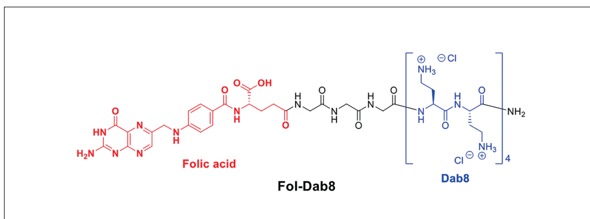
The structure of the artificial cationic peptide (Fol-Dab8)
